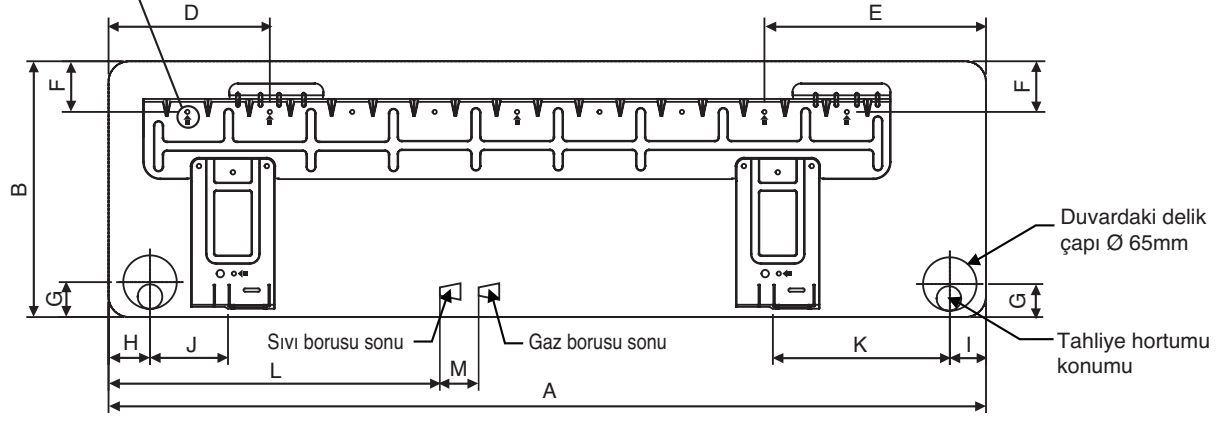
KURULUM LEVHASI FTYN50/60LV1B
