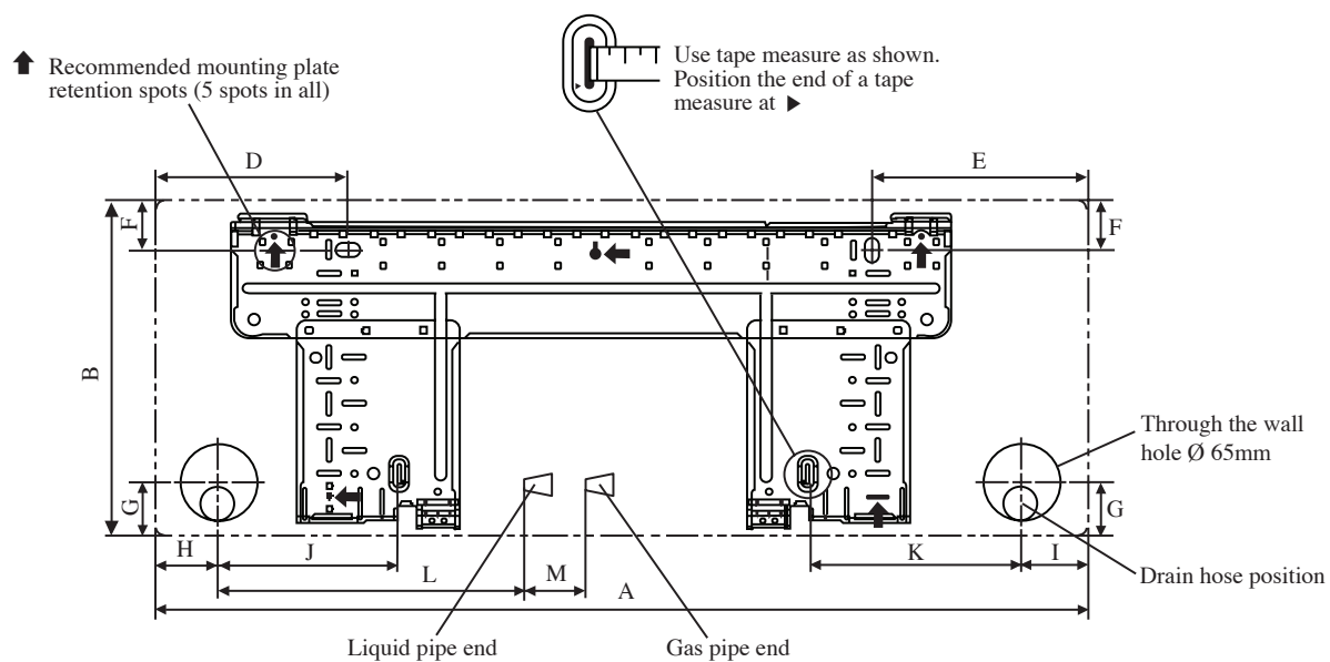
INSTALLATION PLATE FTYN25/35LV1B
