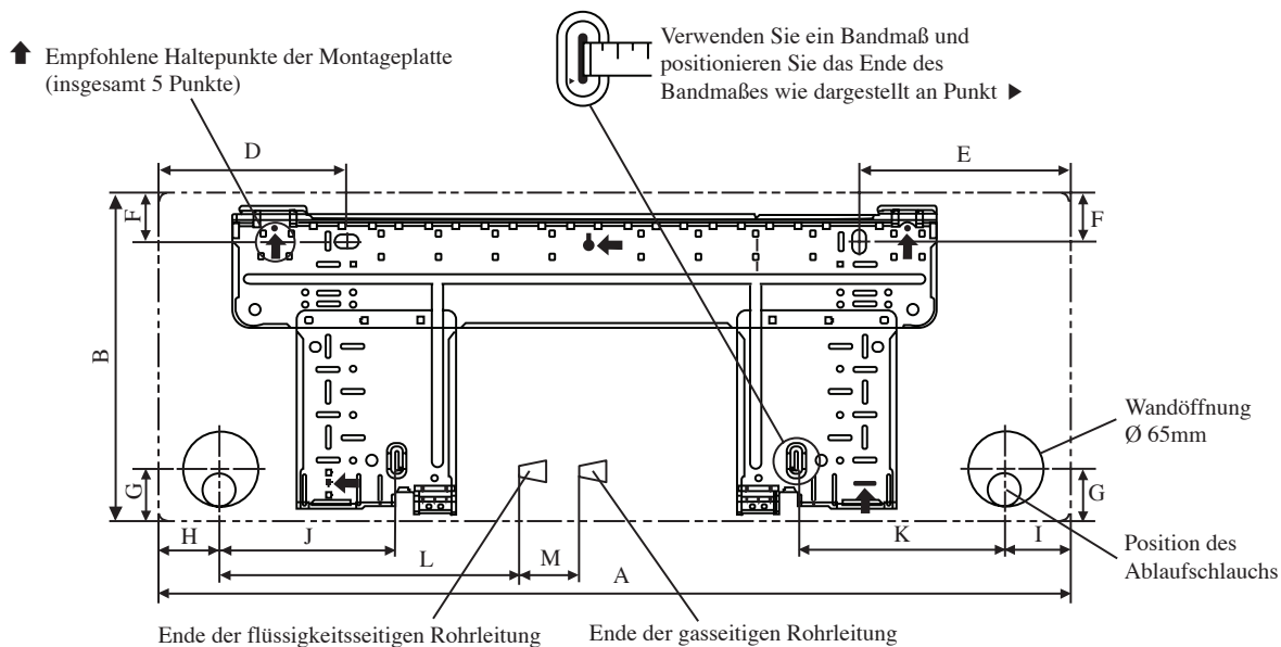
MONTAGEPLATTE FTYN25/35LV1B
